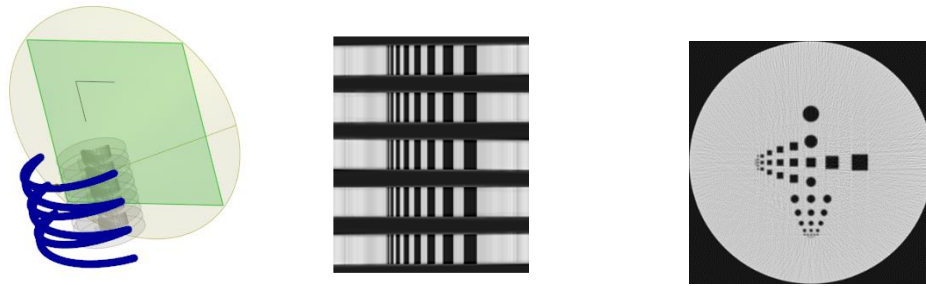
Fig. 5. Reconstruction of the multi-disk phantom using half-scan reverse helical trajectory
